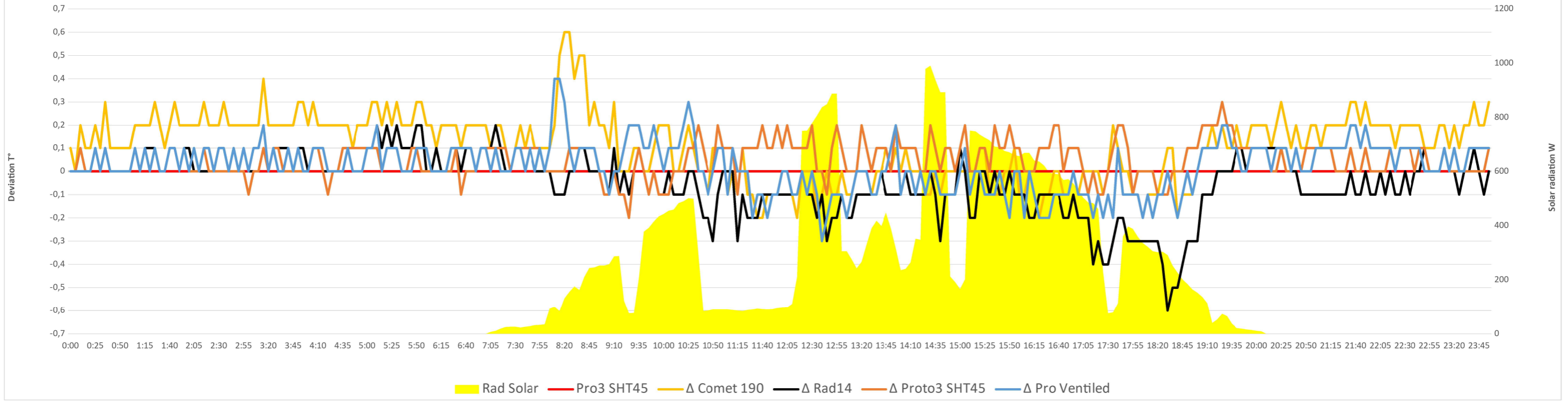
Temperature deviation from reference - with solar radiation
